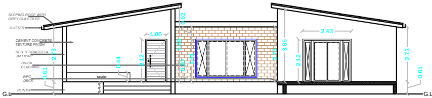
NORTH SIDE ELEVATION (IN FT & IN) SCALE - N.T.S.
