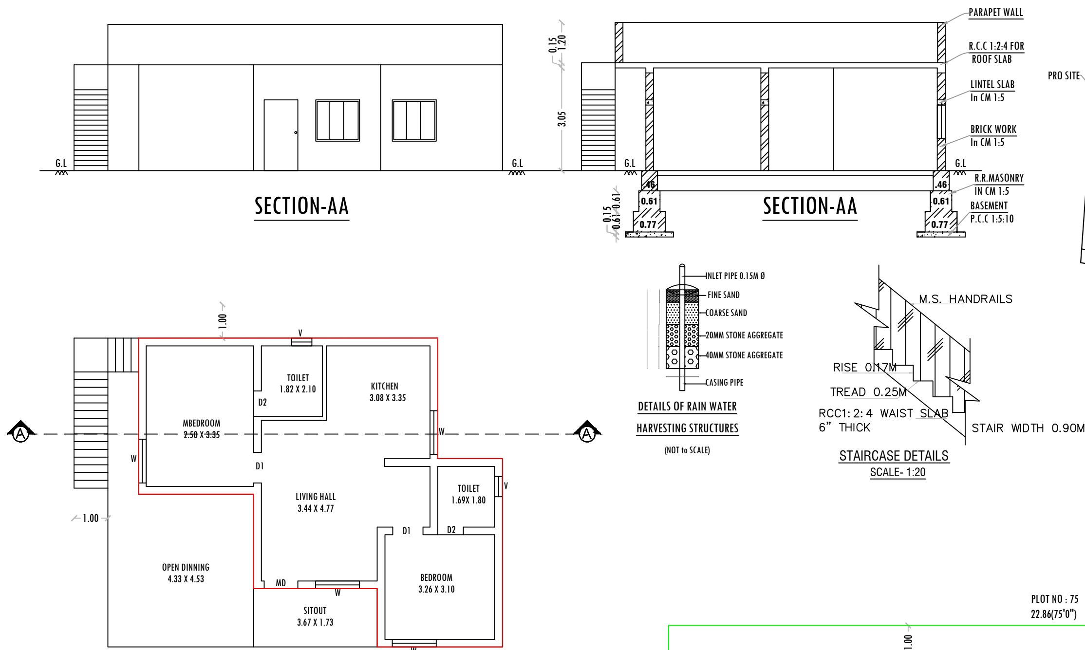
GROUND FLOOR
