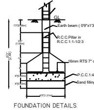
FOUNDATION DETAILS
