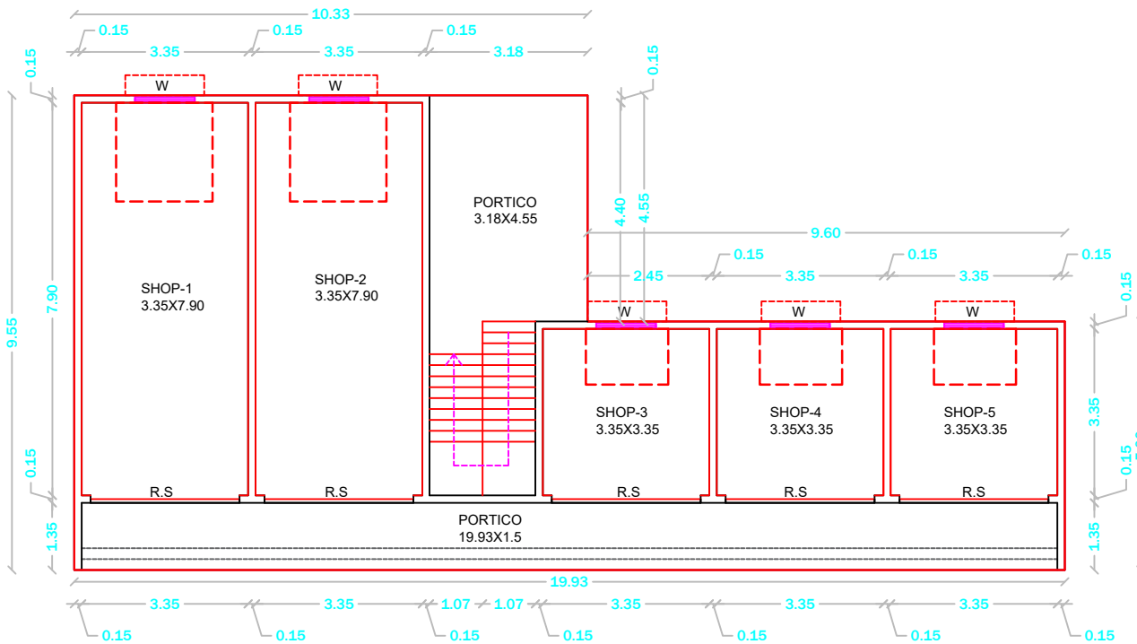
PRO. GROUND FLOOR PLAN COMMERCIAL
