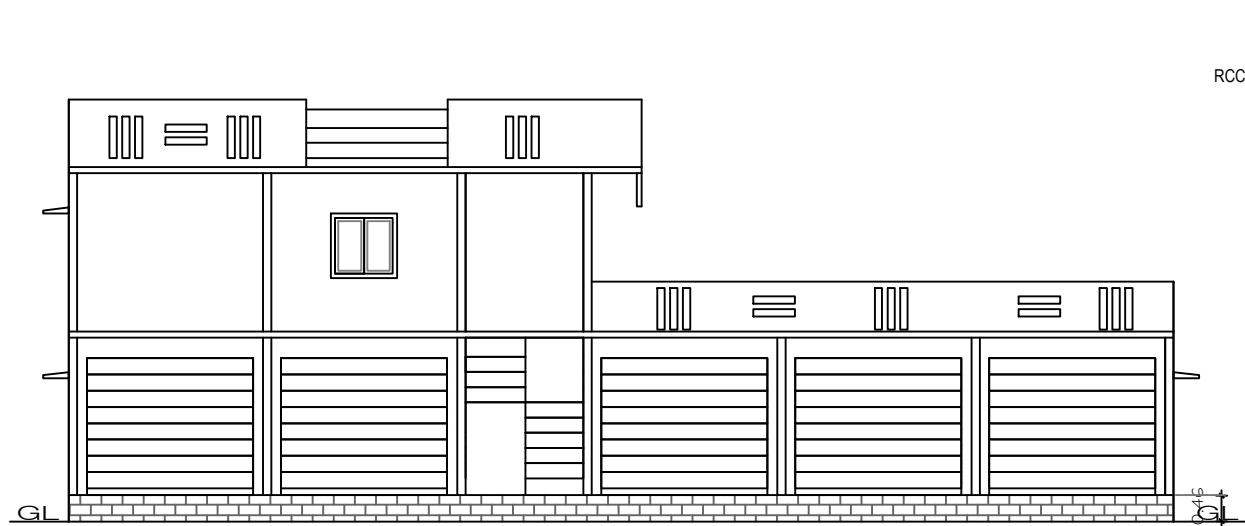
FRONT ELEVATION.
