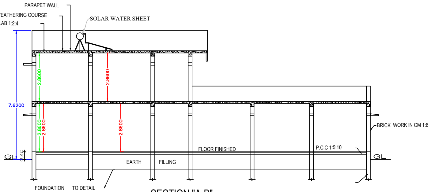
SECTION "A-B"
