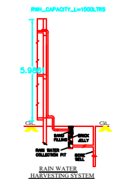
RAIN WATER HARVESTING SYSTEM
