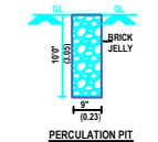
PERCULATION PIT
