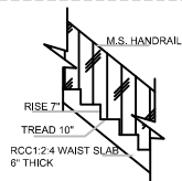
STAIRCASE DETAIL SCALE- 1:20
