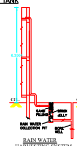
RAIN WATER HARVESTING SYSTEM RWH_CAPACITY_L=1000LTRS
