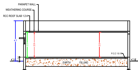
SECTION "A-B"
