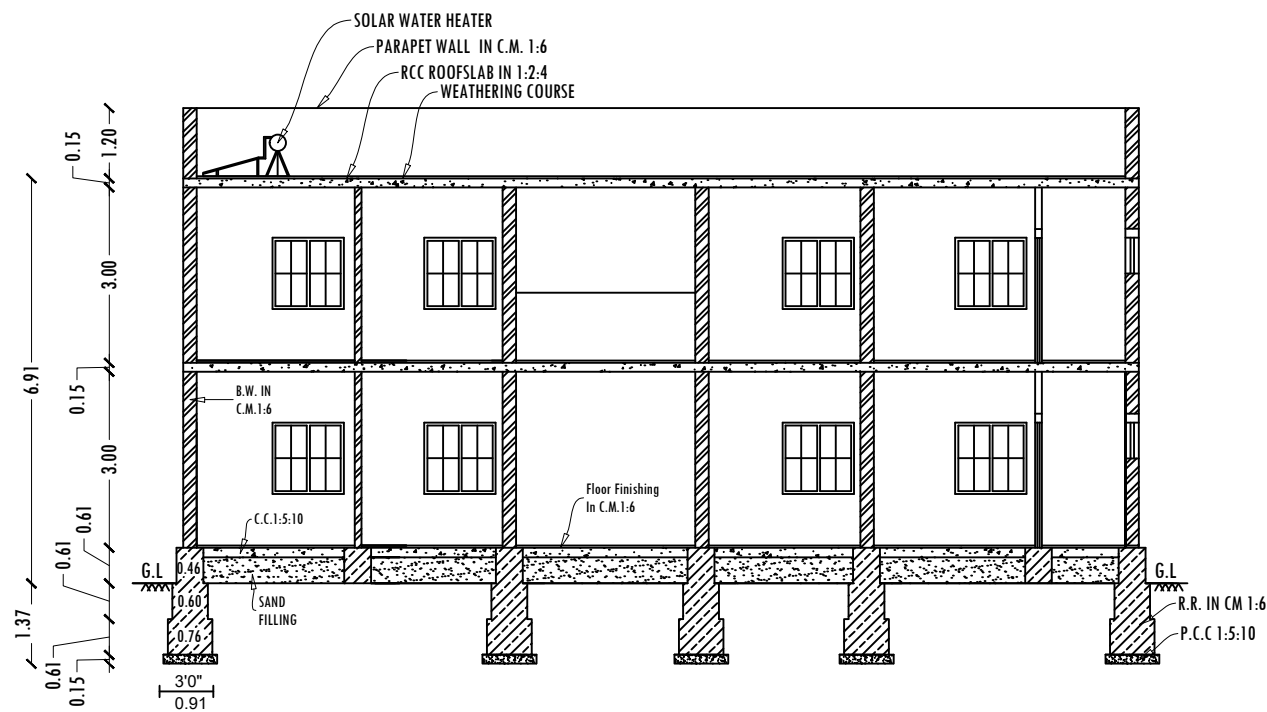
SECTION -AA
