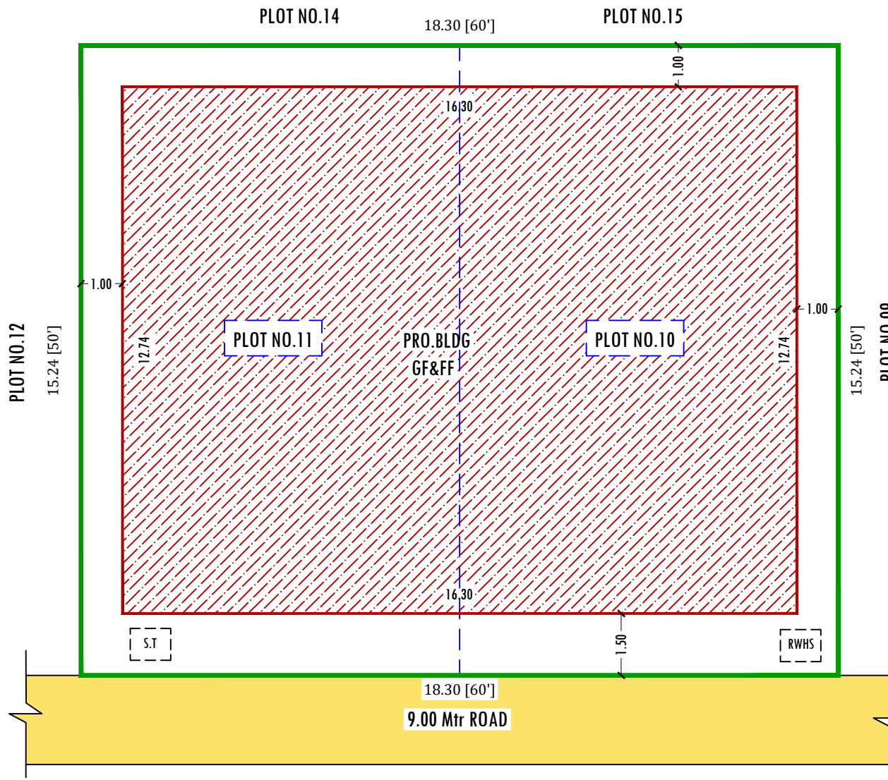
SITE PLAN
