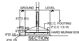
FOUNDATION DETAILS
