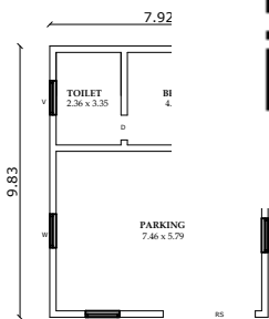
GROUND FLOOR - PARKING
