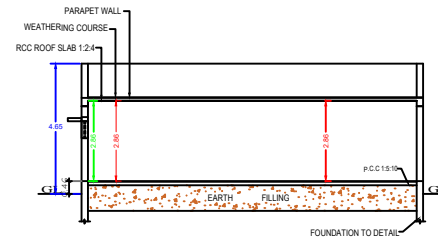
SECTION "A-B"
