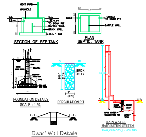
Dwarf Wall Details
