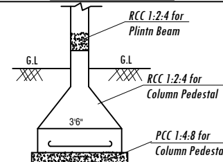
Typical Cross-Section
