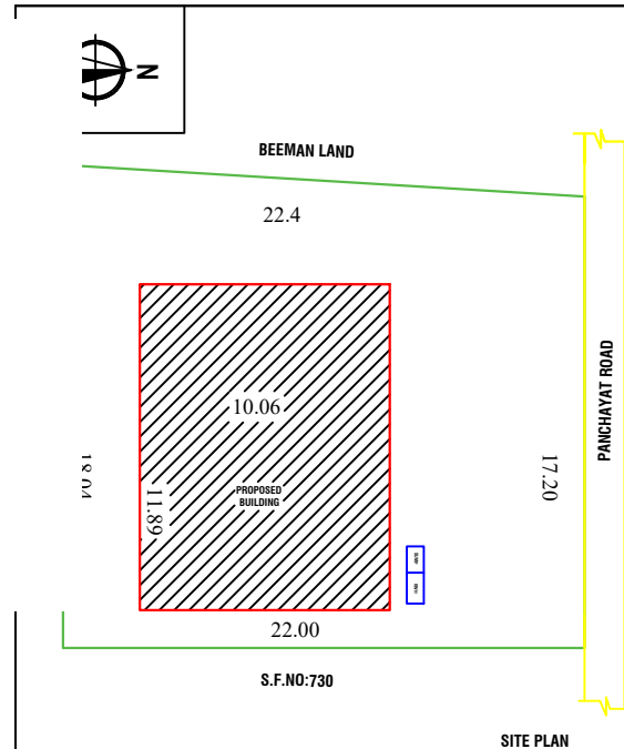
SITE PLAN
