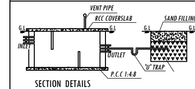
SECTION DETAILS
