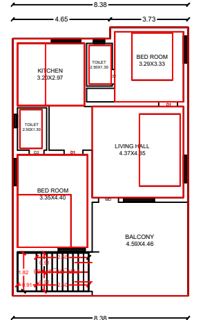
PRO. SECOND FLOOR PLAN.
