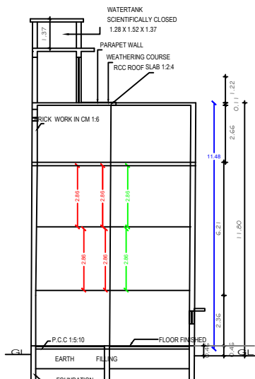
SECTION "A-B"
