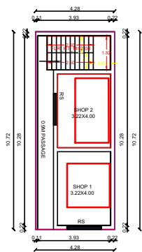
PRO.GROUND FLOOR PLAN SCALE:1:100
