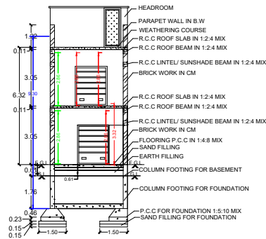
SECTION "A-B"
