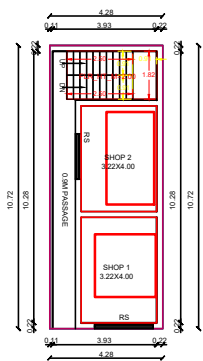
PRO.FIRST FLOOR PLAN SCALE:1:100
