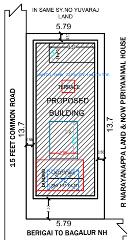
SITE PLAN SCALE:1:100
