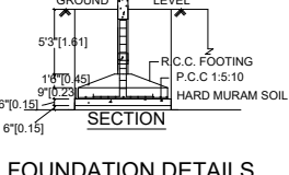
FOUNDATION DETAILS
