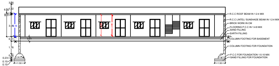
SECTION ON-AA
