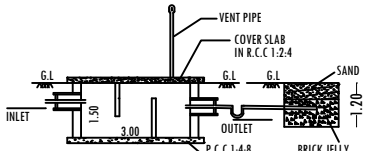
SECTION-AB
