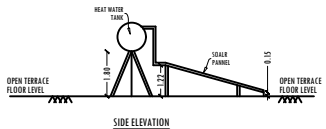
SIDE ELEVATION
