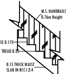
STAIRCASE DETAILS SCALE- 1:20
