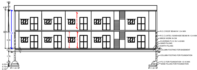
SECTION ON-AA
