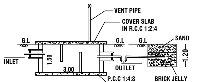
SECTION-AB
