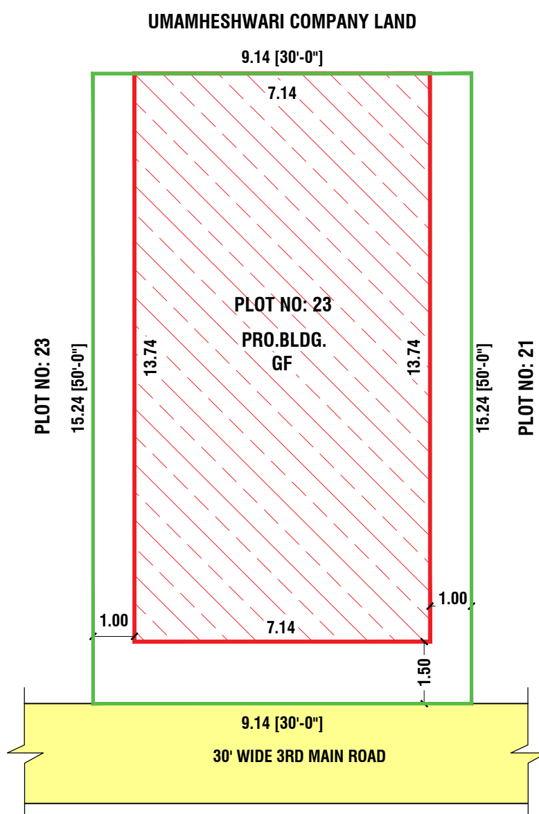
SITE PLAN
