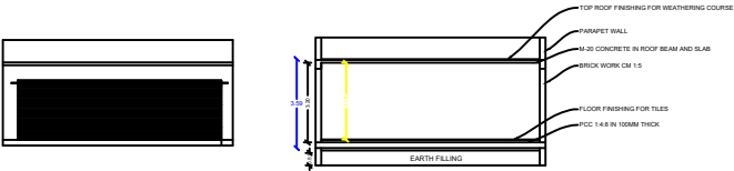
FRONT ELEVATION
