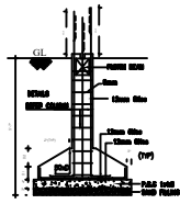
FOUNDATION DETAILS
