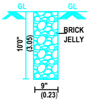
PERCOLATION PIT
