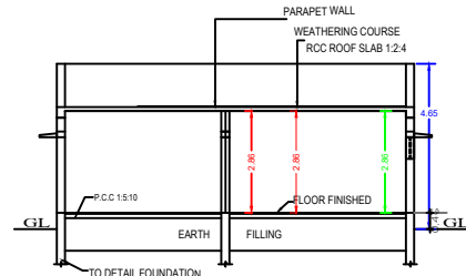
SECTION "A-B"
