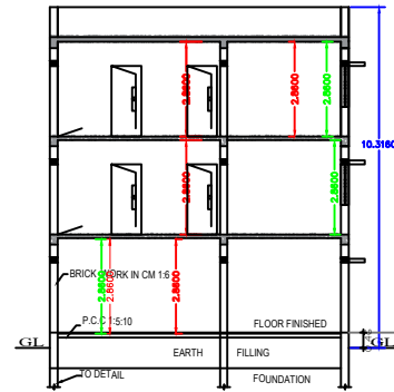
SECTION "A-B"
