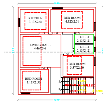
EXI.FIRTS FLOOR PLAN SCALE:1:100
