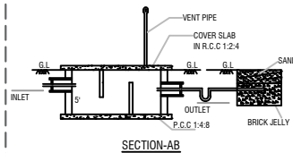
SECTION-AB
