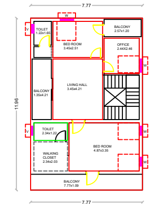
PRO. SECOND FLOOR PLAN SCALE: 1:100
