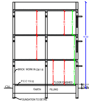
SECTION "A-B"
