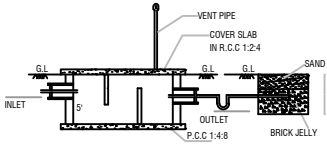
SECTION-AB
