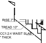
STAIRCASE DETAILS SCALE- 1:20
