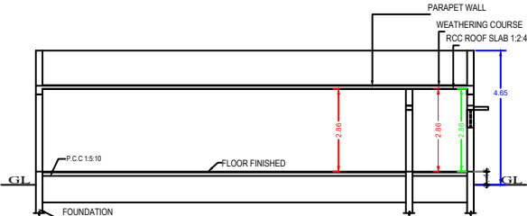
SECTION "A-B"
