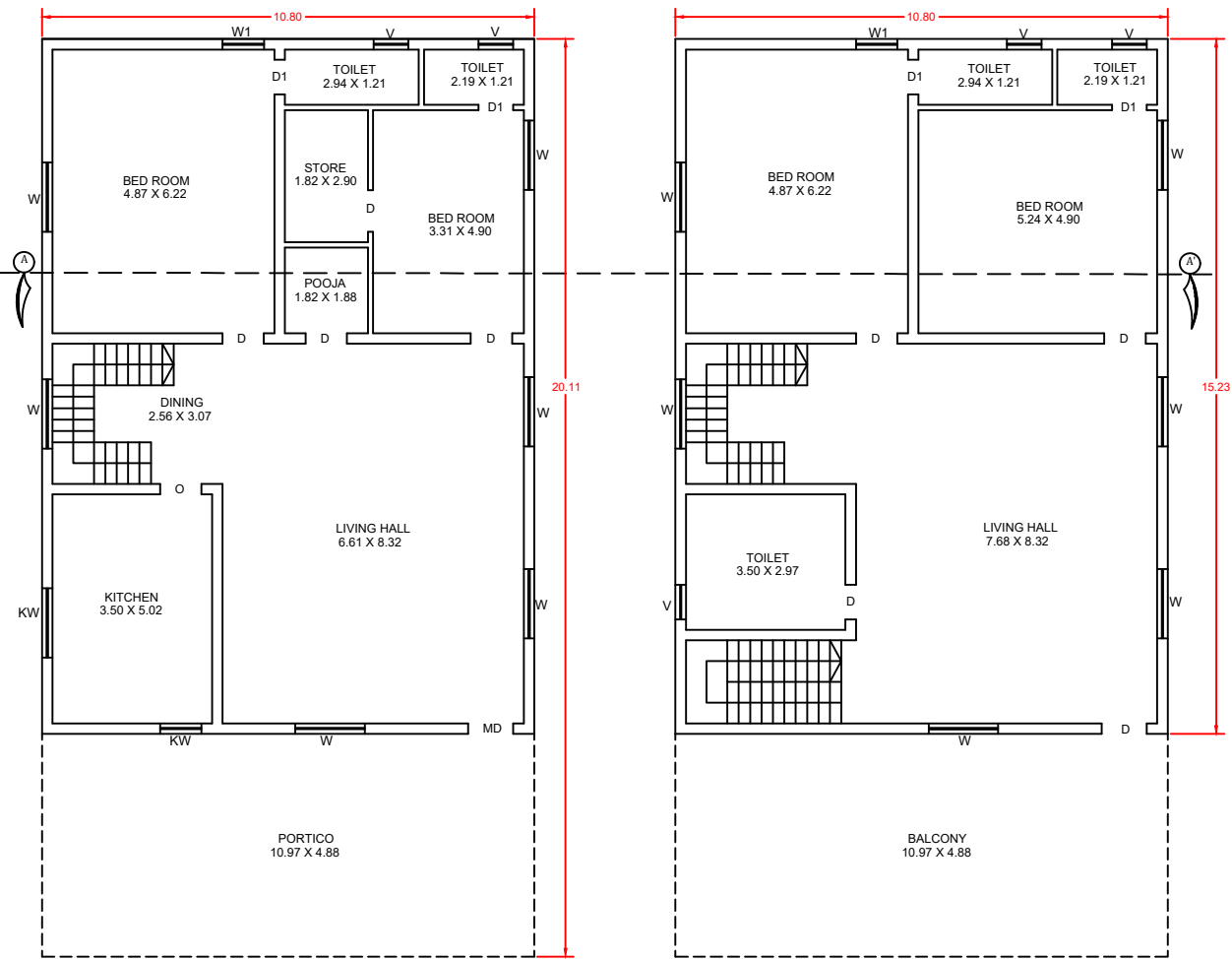
FIRST FLOOR
