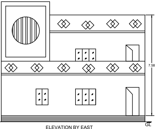
ELEVATION BY EAST
