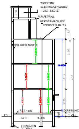
SECTION "A-B"
