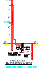
RAIN WATER HARVESTING SYSTEM RWH_CAPACITY_L=1000LTRS
