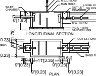
SEPTIC TANK:
