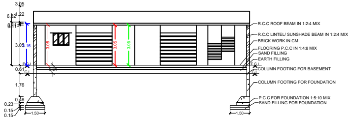
SECTION ON-AA
