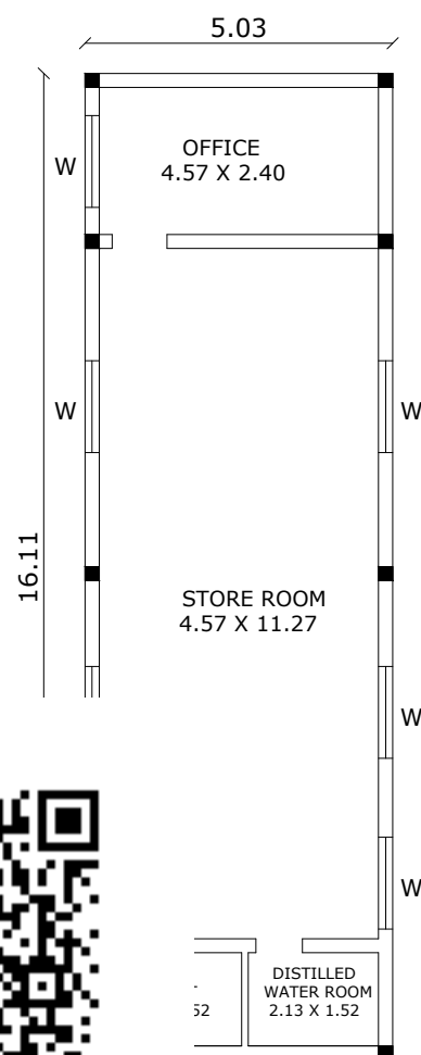
FLOOR PLAN
