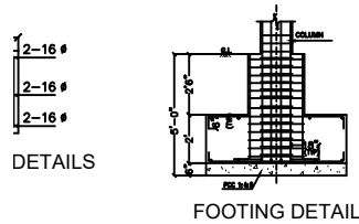
FOOTING DETAIL
