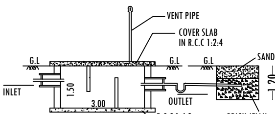
SECTION-AB
