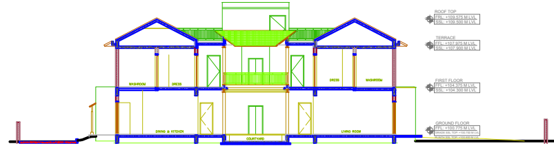
SECTION B
