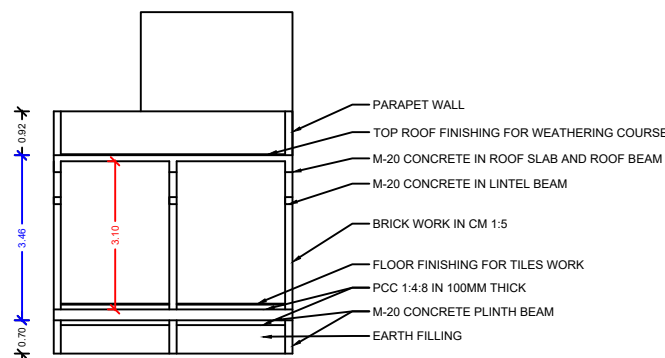
CROSS SECTION
