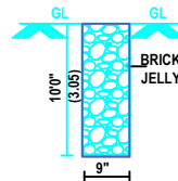
PERCOLATION PIT
