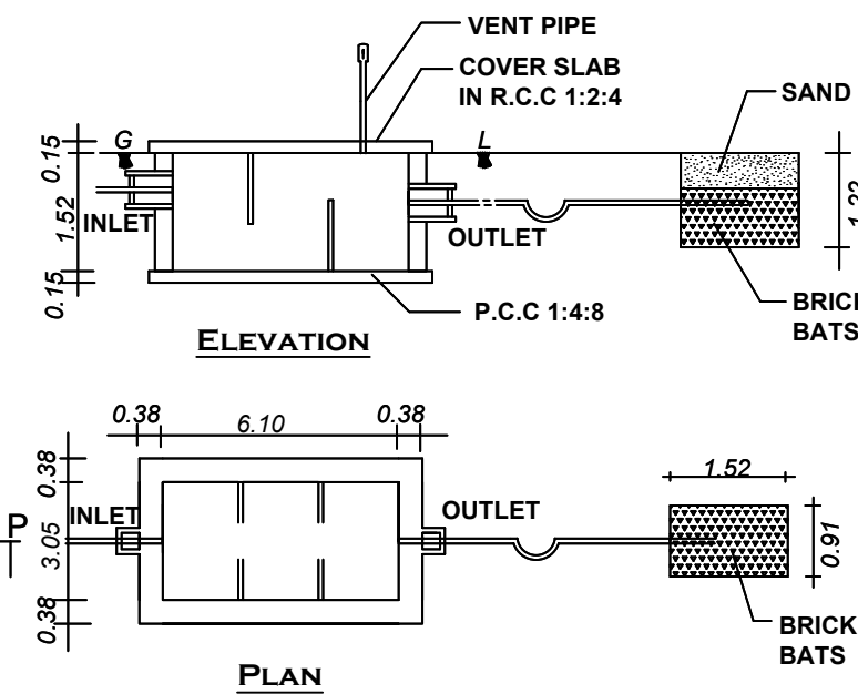
SEPTIC TANK & DISPERSION TRENCH DETAILS
