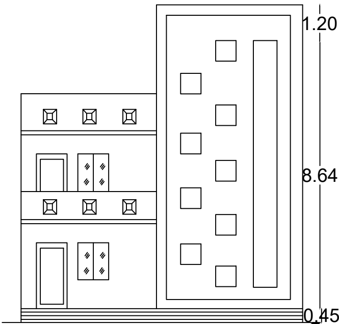
ELEVATION BY NORTH
