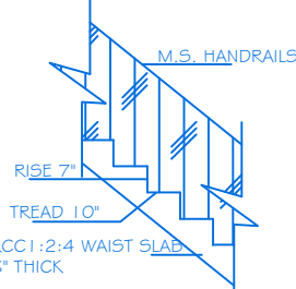
STAIRCASE DETAILS SCALE- 1:20
