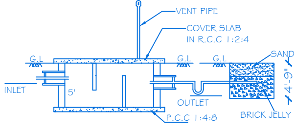
SECTION-AB
