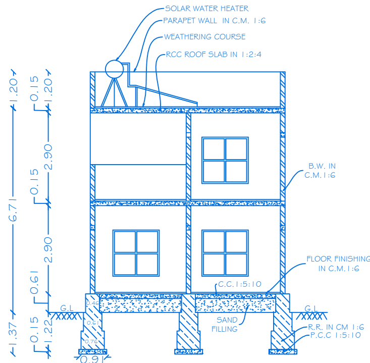
SECTION ON-AA
