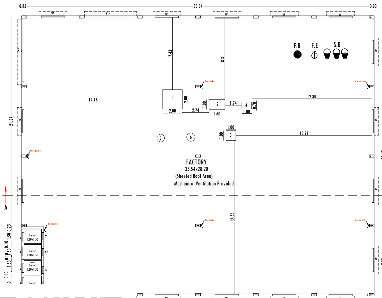
GROUND FLOOR (BLOCK-1)
