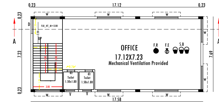
GROUND FLOOR (BLOCK-2)
