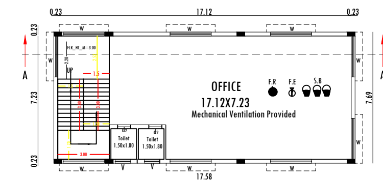
FIRST FLOOR (BLOCK-2)
