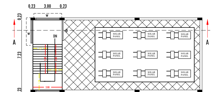
TERRACE FLOOR (BLOCK-2)
