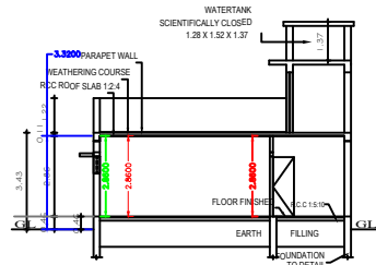
SECTION "A-B"
