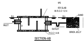
SECTION-AB
