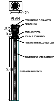
PERCOLATION PIT
