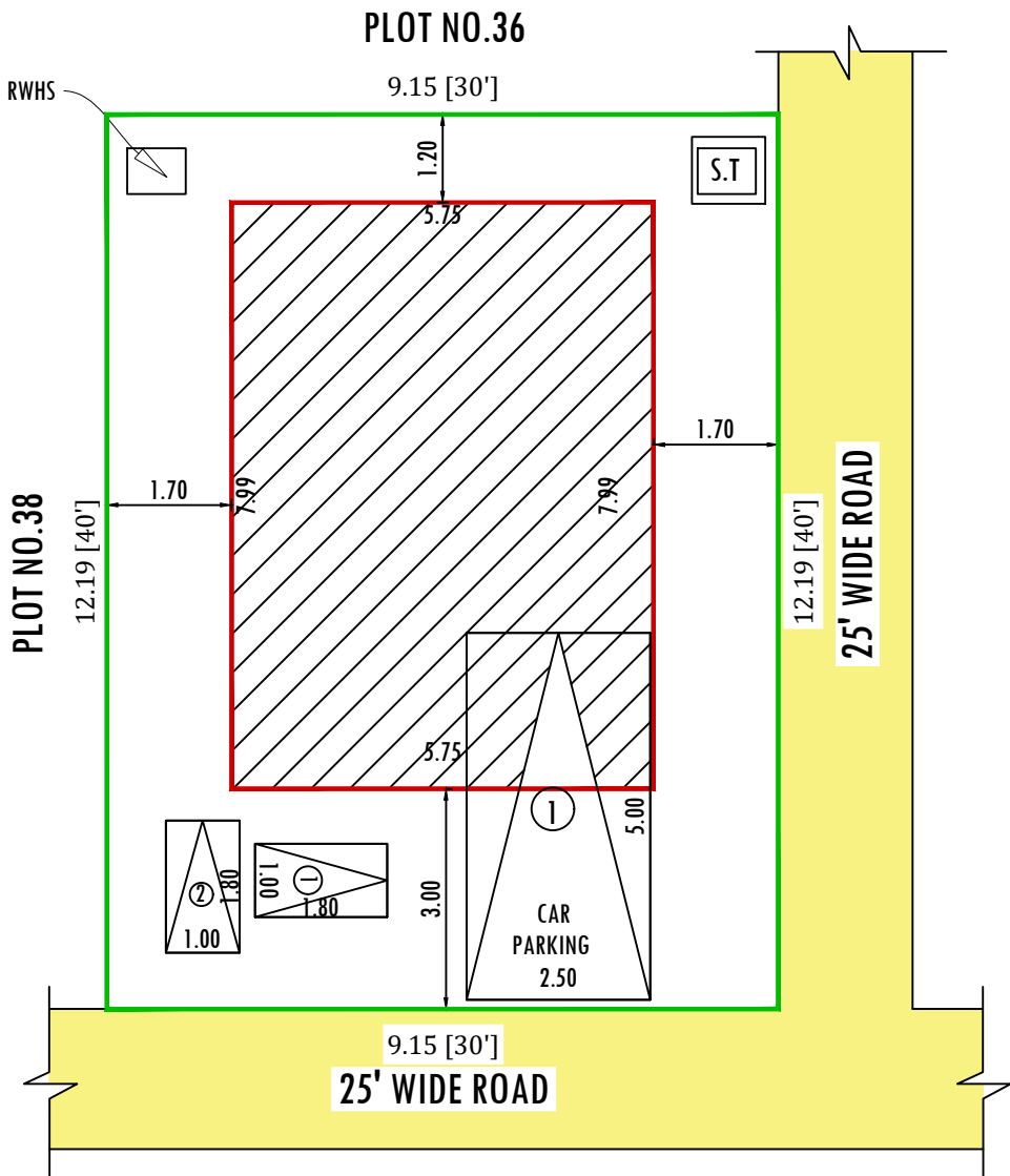
SITE PLAN
