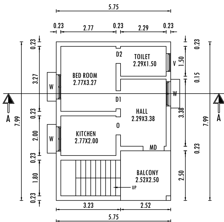
PRO.SECOND FLOOR
