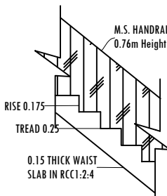
STAIRCASE DETAILS
