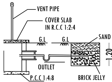
SECTION-AB
