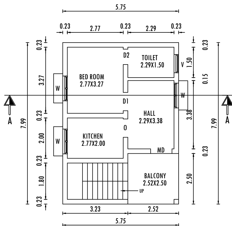
EXG.FIRST FLOOR
