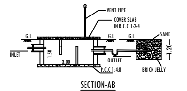
SECTION-AB
