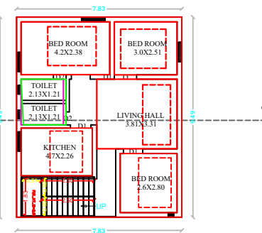
PRO.SECOND FLOOR PLAN SCALE:1:100
