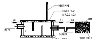
SECTION-AB
