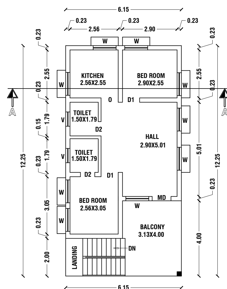
PRO. SECOND FLOOR PLAN
