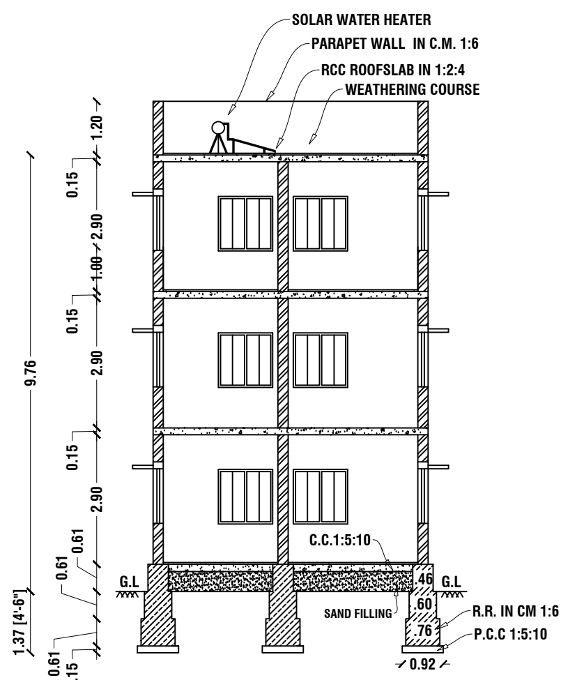
SECTION -AA
