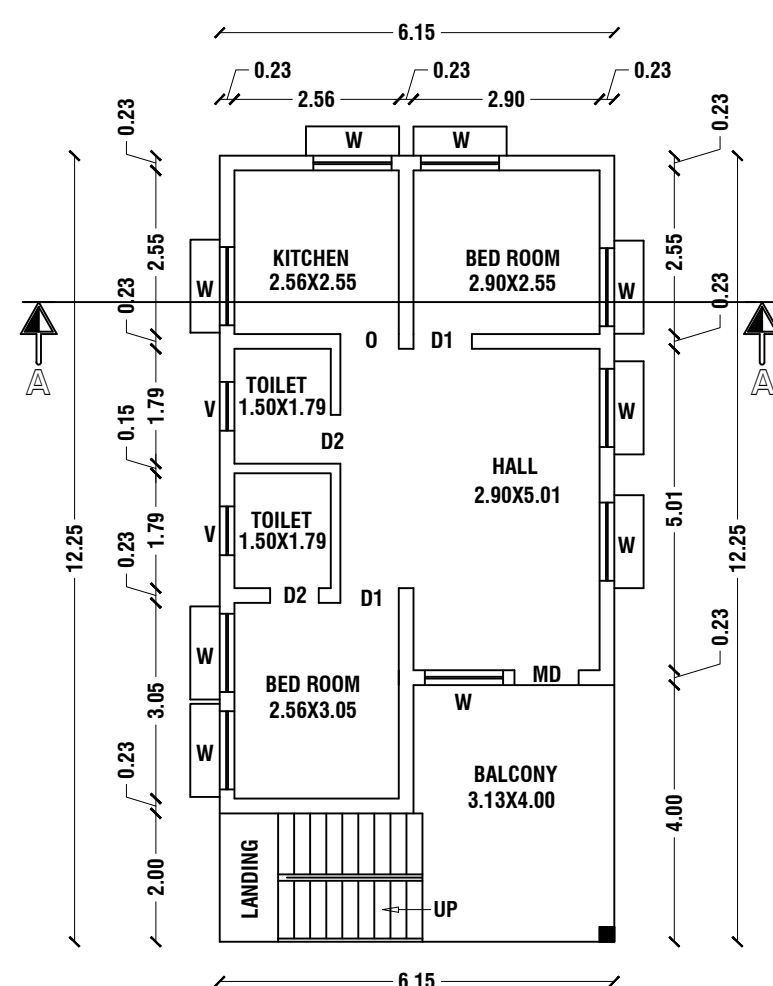
EXG. FIRST FLOOR PLAN
