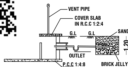
SECTION-AB
