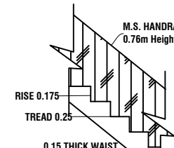
STAIRCASE DETAILS SCALE- 1:20
