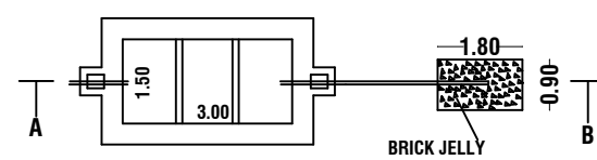
SEPTIC TANK & DISPERSION TRENCH DETAILS
