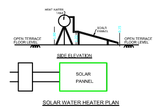
SOLAR WATER HEATER PLAN
