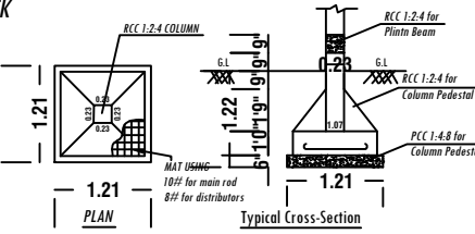
FOOTING DETAILS
