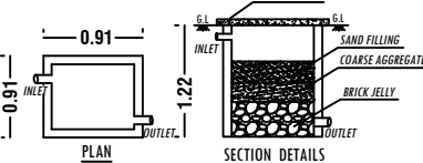
RAINWATER HARVESTING SYSTEM
