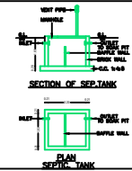
PLAN SEPTIC TANK
