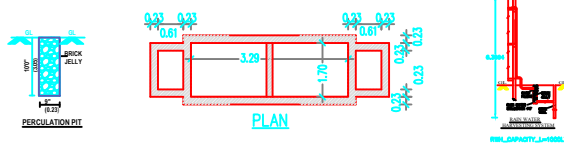
FOUNDATION DETAILS SCALE : 1:50.
