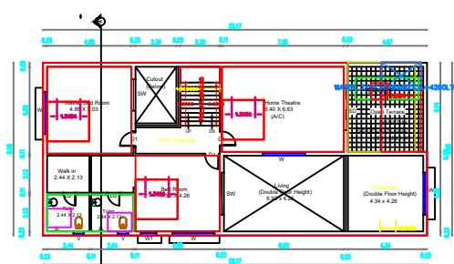
PRO. FIRST FLOOR PLAN.
