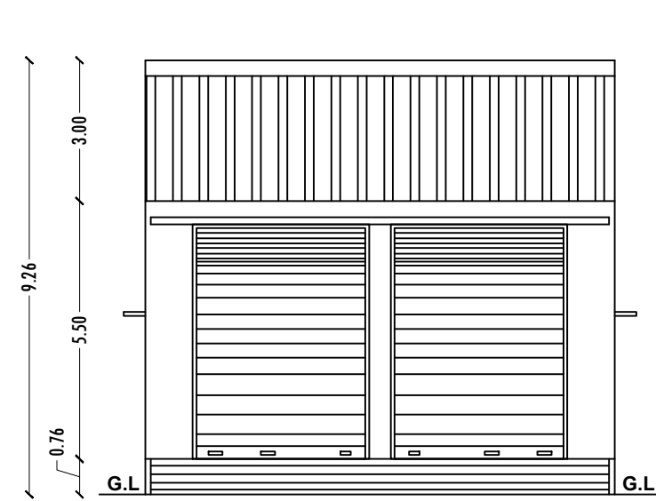
FRONT ELEVATION
