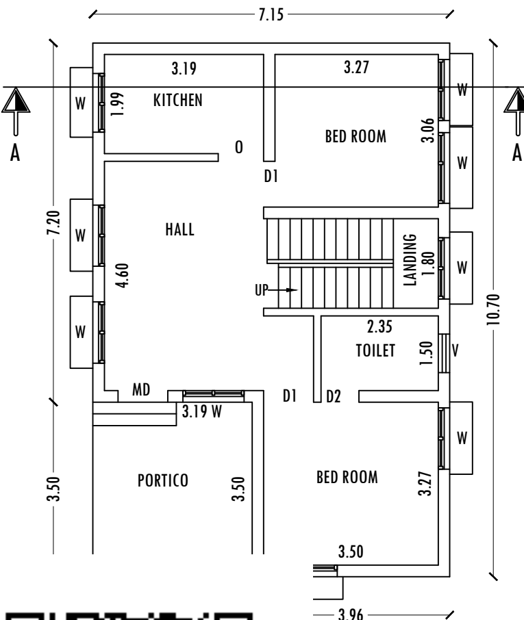
FLOOR PLAN
