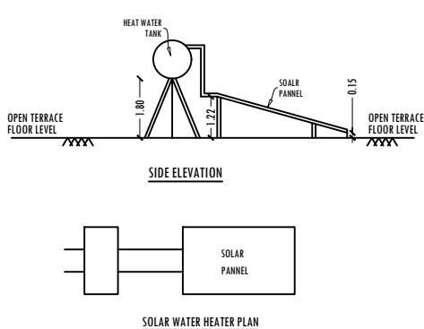
SOLAR WATER HEATER PLAN
