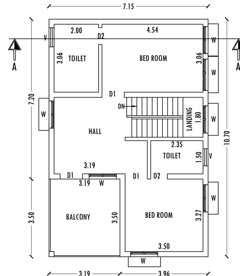
EXTG-FIRST FLOOR PLAN
