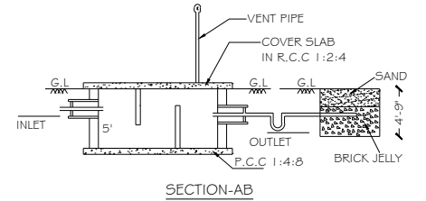
SECTION-AB
