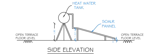
SIDE ELEVATION
