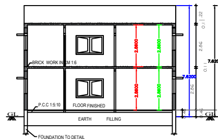
SECTION "A-B"
