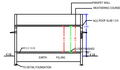
SECTION "A-B"
